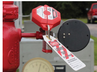
Gate Valve Handle Lockouts 10K123 For 2-1/2" - 5" handle
