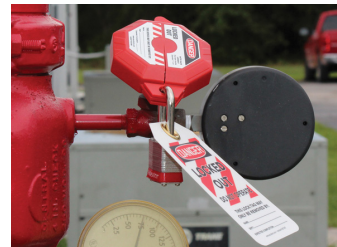
Gate Valve Handle Lockouts
